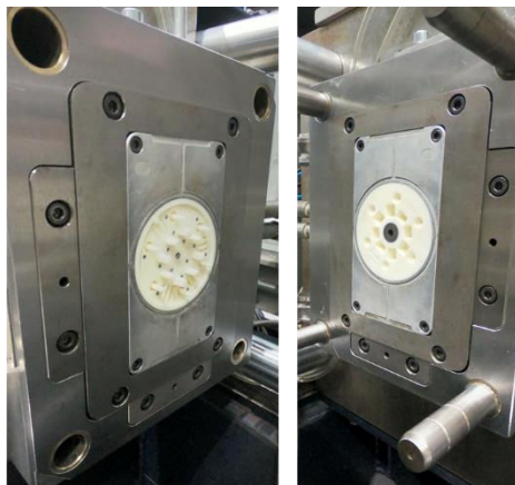
3D-printed insert in base mold
