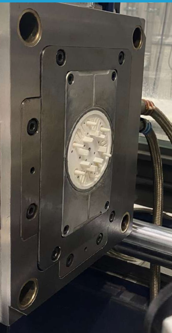
3D printed tool insert Image © DREIGEIST
